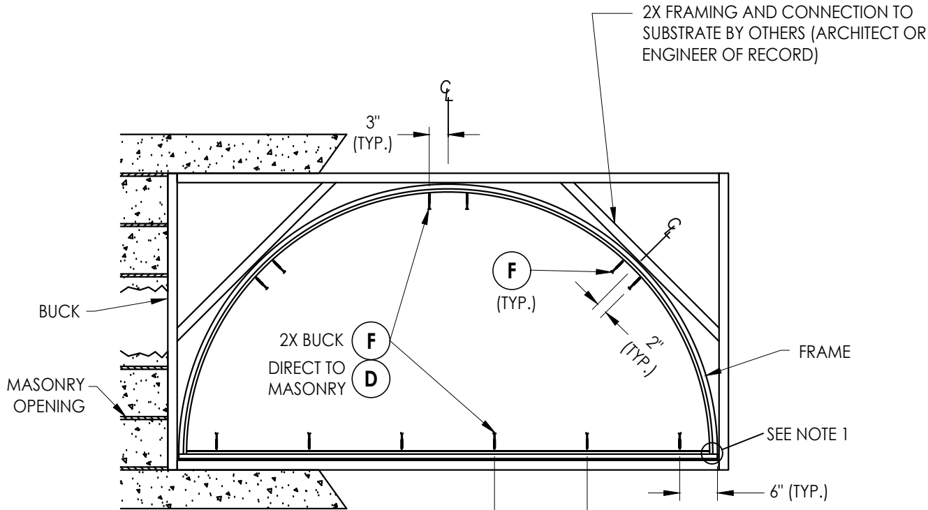
FRAME ANCHORING HALF-ROUND
